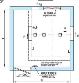
机房平面图 plane layout of machine room
